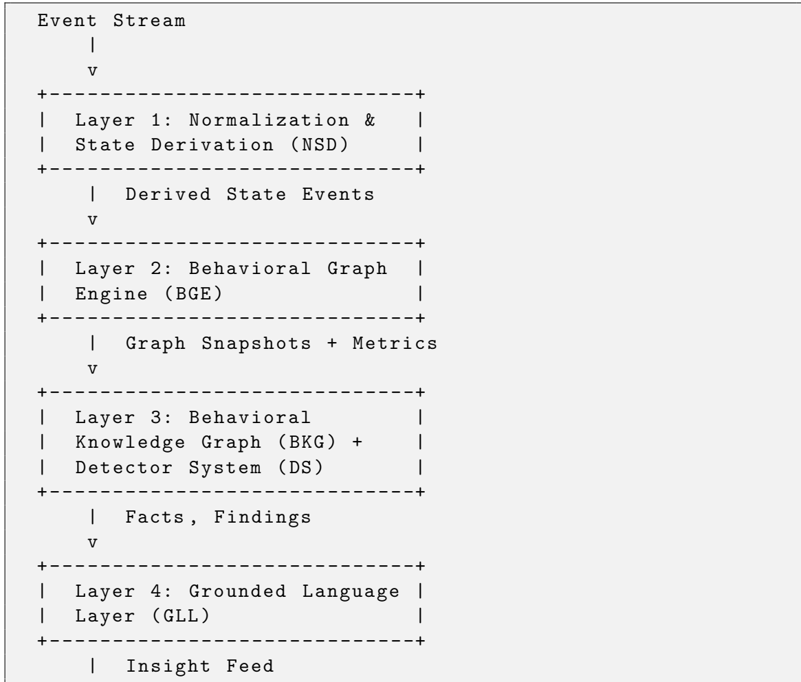
Figure 1: BIP data flow. Each layer produces a structured artifact consumed by the next.
