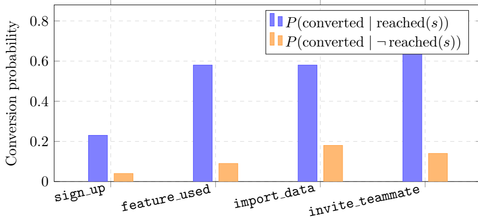
Figure 3: Absorption probabilities B (Eq. (4)) computed from synthetic simulation data. Blue bars show the probability of conversion given the user visited state s ; orange bars show conversion probability among users who never visited s . Note that import_data achieves a lift of 0.58/0.18 \approx 3.2\times , consistent with the fact bundle example in Section 7.
