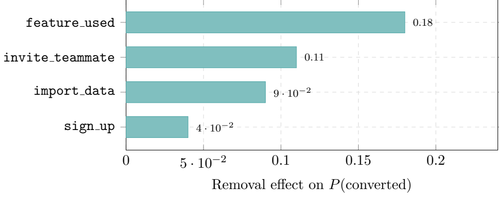
Figure 4: Removal effect ranking (Eq. (8)) for the example funnel. Each bar shows the decrease in overall P(\text{converted}) when the corresponding state is removed from the journey graph and transition probabilities are re-normalised. feature_used is the structurally most critical state, making it the top-ranked activation driver candidate.
