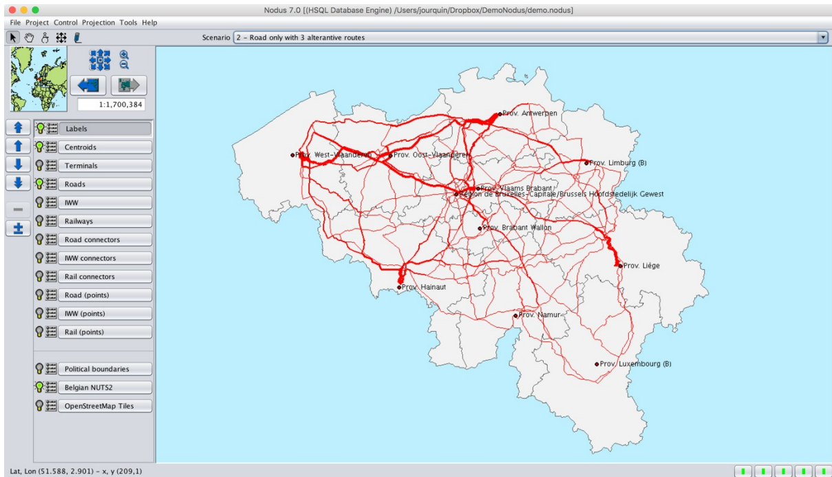
Figure 20: Multi-flow assignment for road transport
