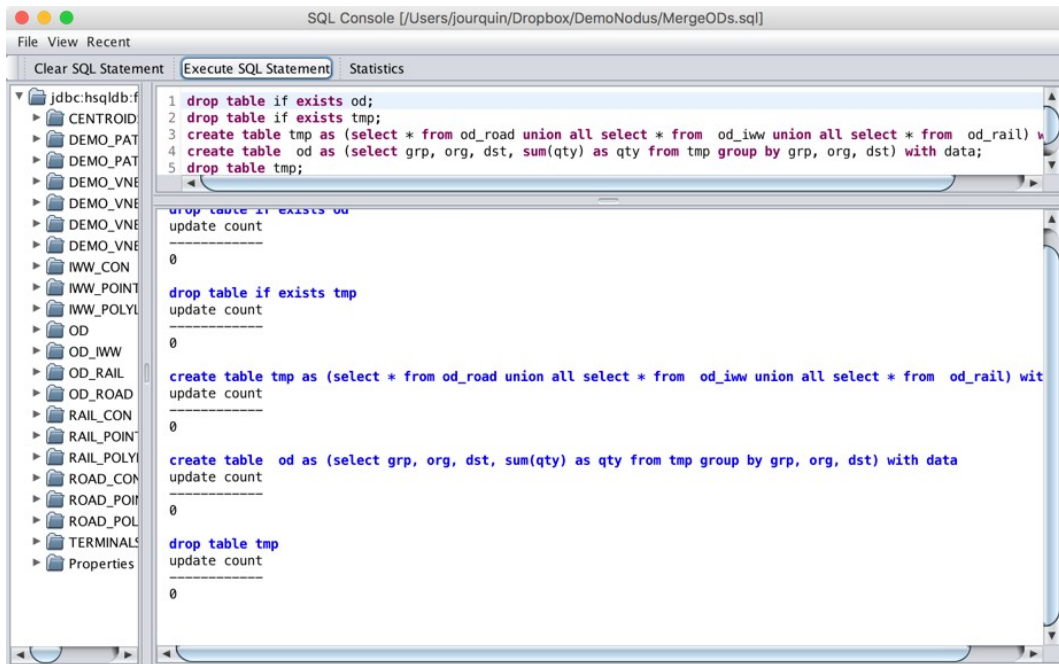
Figure 28: The "MergeODs.sql" script in the SQL Console
