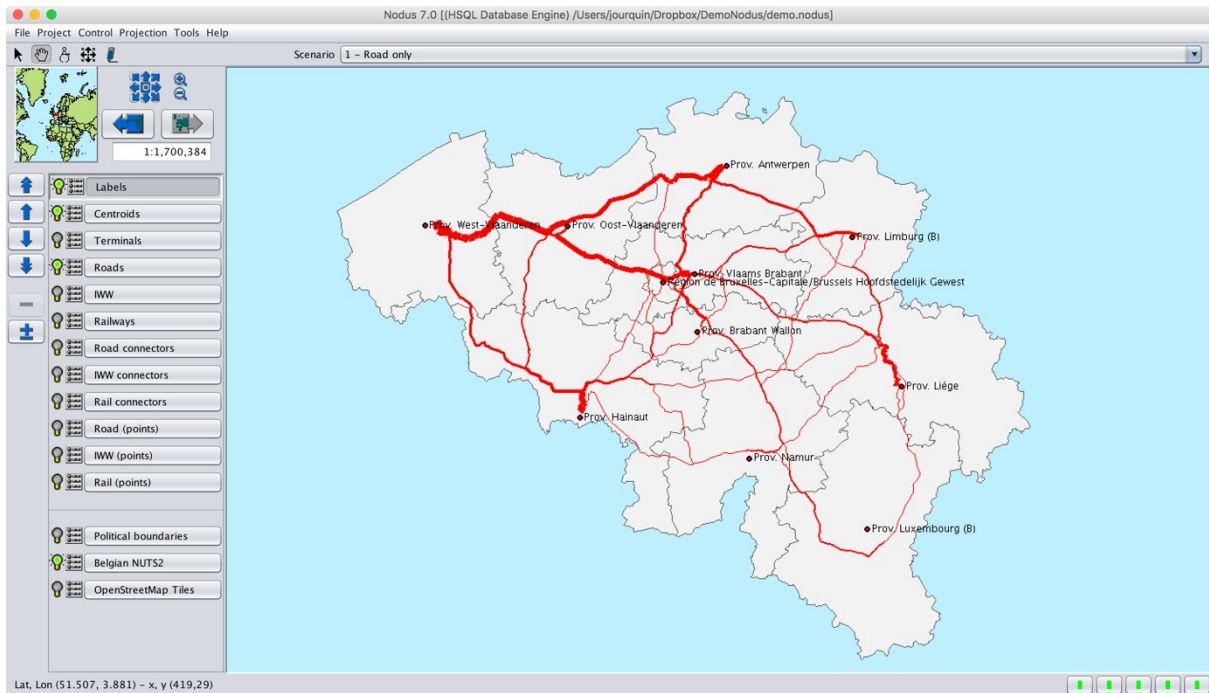
Figure 16: Assignment of scenario 1
