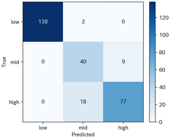
3-bin Speed Probe Confusion
