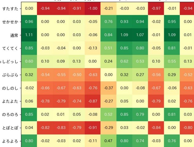
H1 vs HOYO Margin Matrix (Centered Cos) M[i,j] = S[i,i] - S[i,j] (Row: H1 style, Col: HOYO style)
