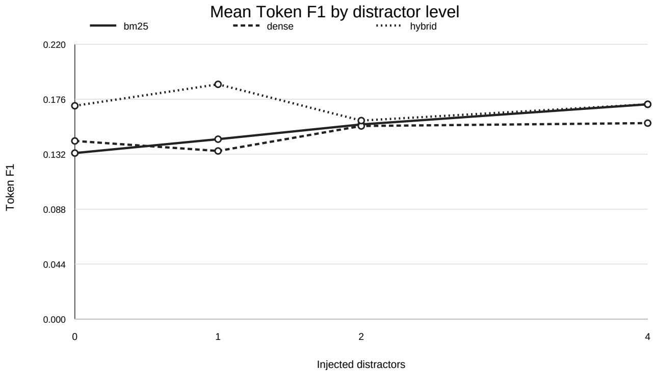
Mean Token F1 by distractor level
