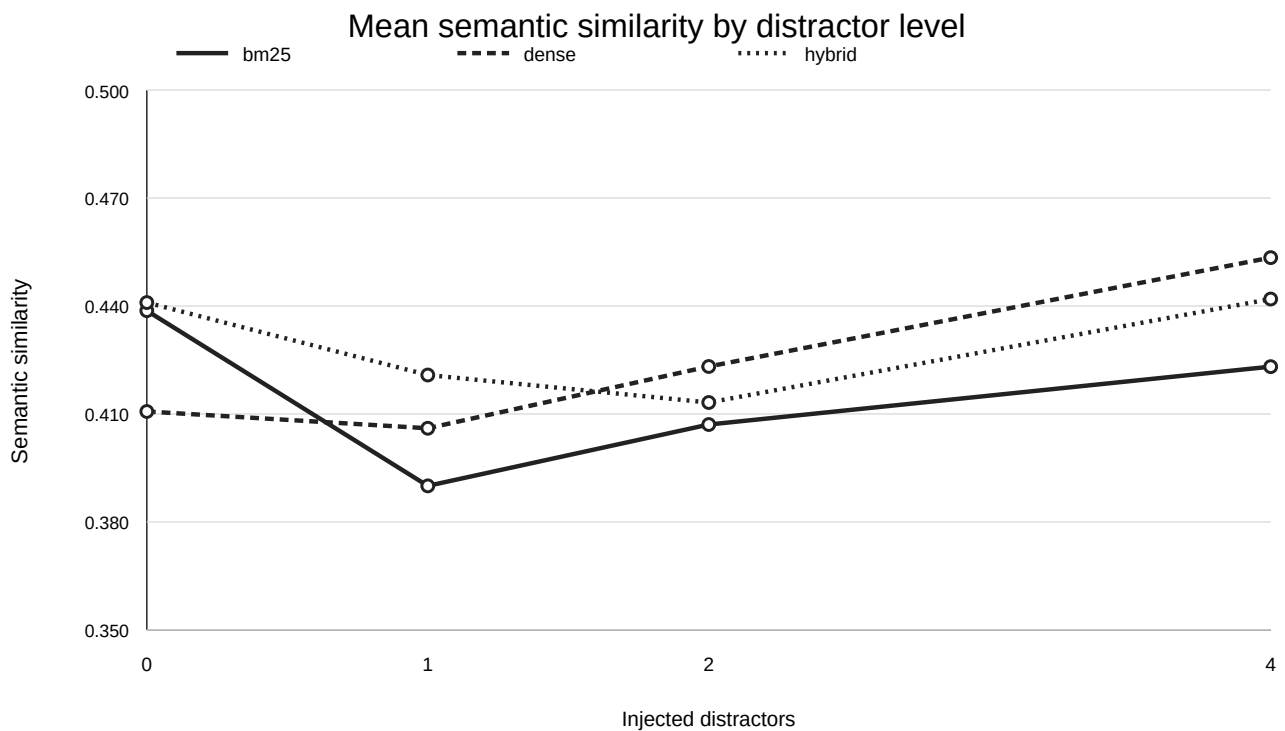
Mean semantic similarity by distractor level
