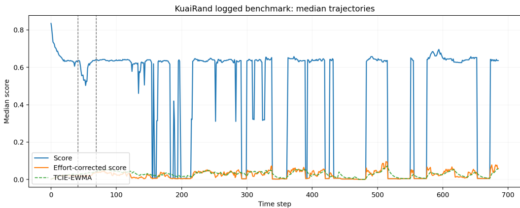
Figure 6: KuaiRand logged benchmark. The random-exposure phase is treated as healthy, the first half of the later standard-recommendation slice as bubble formation, and the second half as collapse. Thresholds for \mathcal{C} , \mathcal{C}^E , and EWMA-smoothed \mathcal{C}^E are calibrated only on healthy windows.
