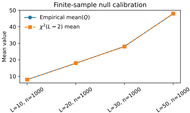
Figure 1: Finite-sample null calibration of the residual-based adequacy statistic.
