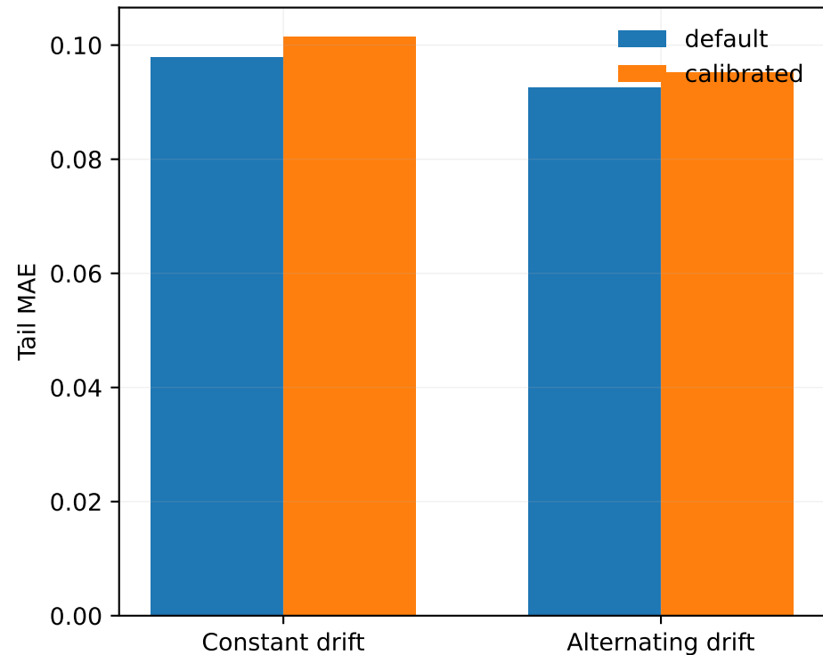
Prefix-validated calibration
