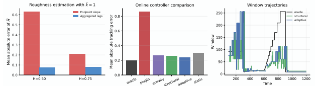
Figure 8: Embedded geometry and online adaptation. Left: TwoNN recovers the intrinsic regime and aggregated lag statistics estimate H far more accurately than endpoint slopes. Middle: the structural controller improves decisively on the naive plug-in rule and beats the activity and static baselines, although the broader validation-based adaptive hybrid remains stronger. Right: the structural controller tracks the contraction and expansion of the oracle window on the default phase profile.
