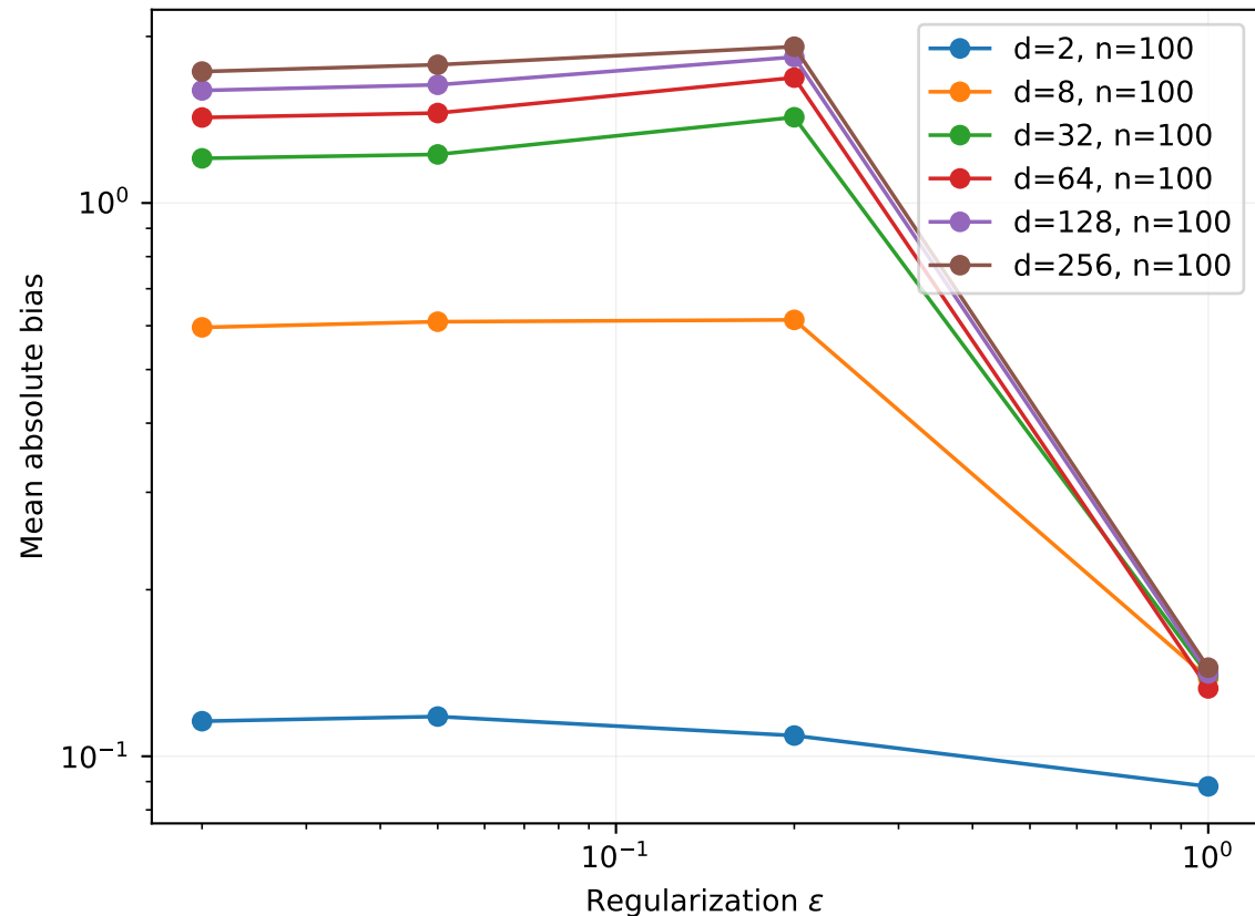
Bias vs regularization
