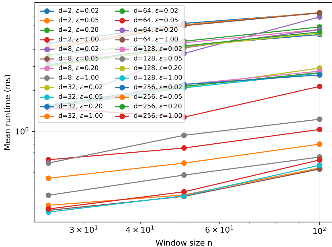
Sinkhorn runtime scaling
