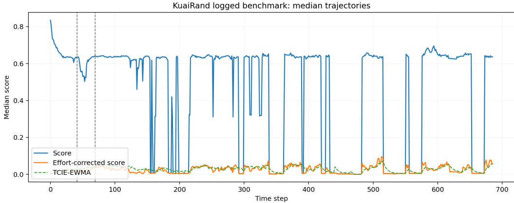
Figure 11: KuaiRand proxy-level logged benchmark. The random-exposure phase is treated as healthy, the first half of the later standard-recommendation slice as bubble formation, and the second half as collapse. Thresholds for CI, CI^E , and EWMA-smoothed CI^E are calibrated only on healthy windows.
