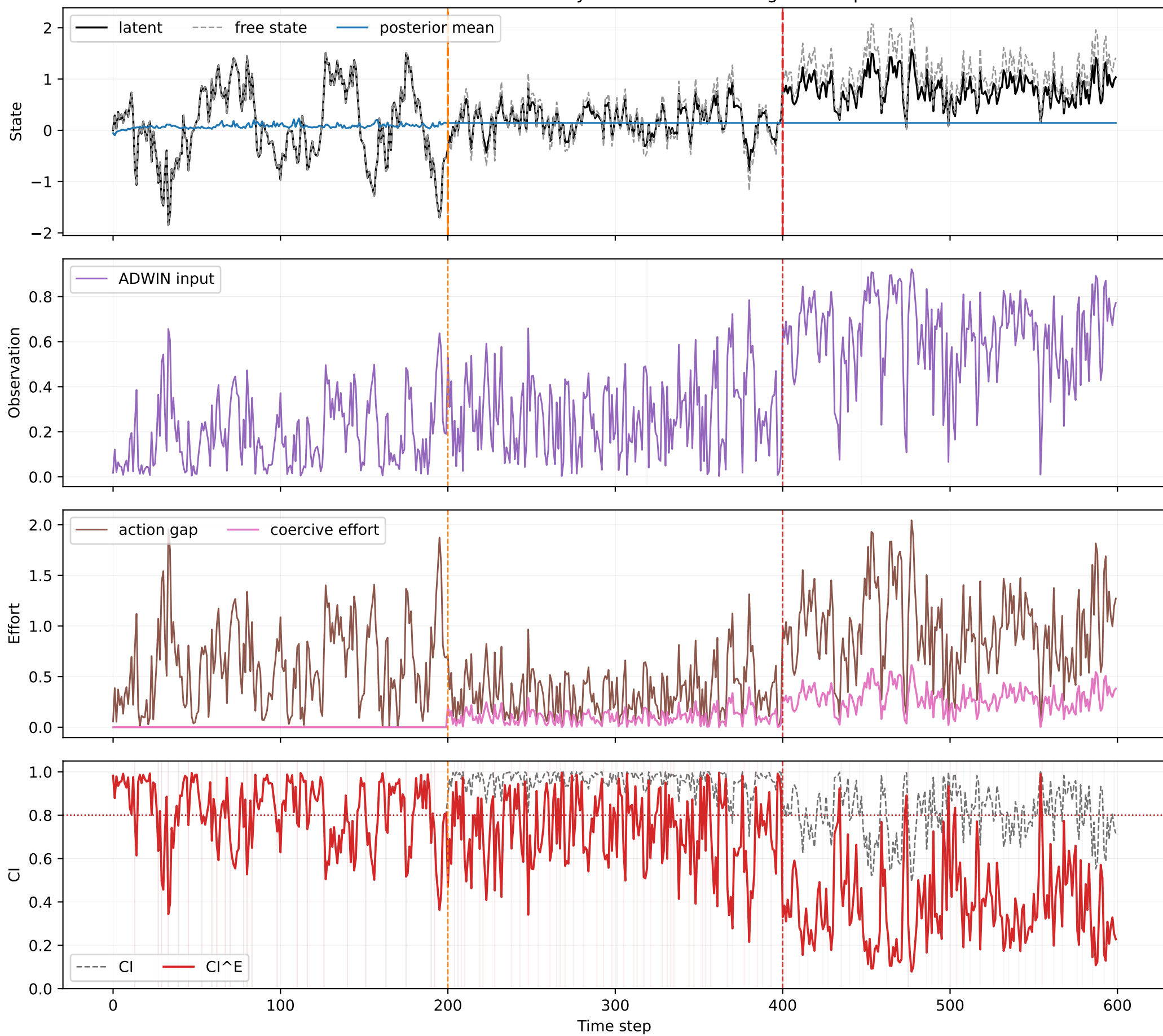
Active benchmark: healthy -&gt; coercive masking -&gt; collapse
