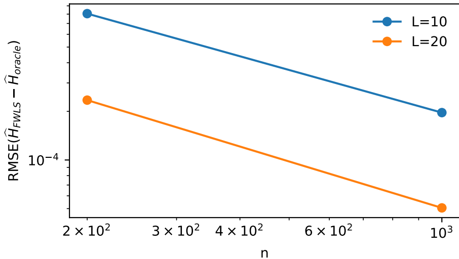
FWLS-oracle agreement
