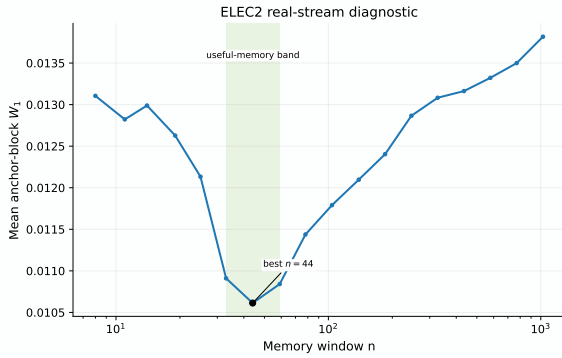
Figure 5: ELEC2 real-stream diagnostic on the nswwprice marginal. The mean anchor-block W_1 error exhibits a finite interior optimum and a near-optimal useful-memory band. The figure is diagnostic: it asks whether the temporal-validity signature appears on a real stream.
