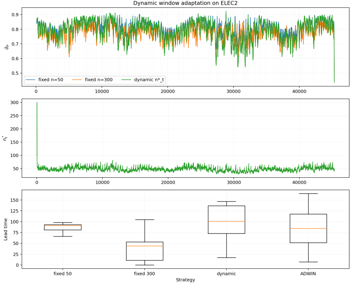
Figure 5: Dynamic n_t^* optimization on ELEC2 ( C_K \approx 1.25 |\bar{s}_t - \bar{s}| \sqrt{100} , EMA \alpha = 0.03 , drift window d = 24 ). Top : \hat{\sigma}_P (100-step mean) for all three strategies; grey lines are PH regime shifts. Middle : dynamic window size n_t^* , contracting sharply near regime shifts and expanding during stable periods. Bottom : lead-time distributions, including the ADWIN baseline.
