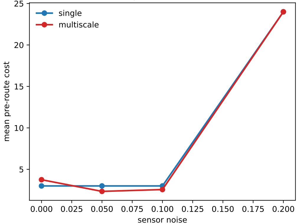
Pre-routing Cost vs Sensor Noise
