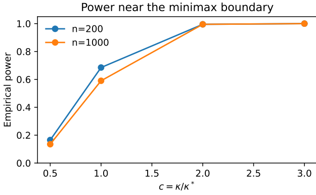
Figure 2: Power transition at the minimax boundary.
