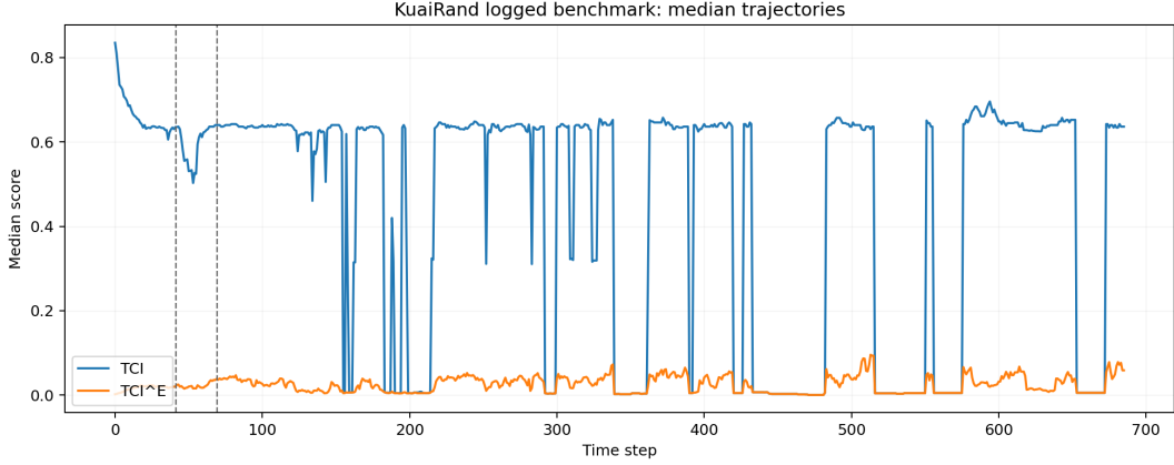
Figure 11: KuaiRand logged benchmark. The random-exposure phase is treated as healthy, the first half of the later standard-recommendation slice as bubble formation, and the second half as collapse. Thresholds for \mathcal{C} and \mathcal{C}^E are calibrated only on healthy windows.
