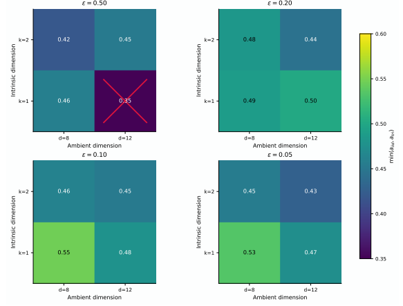
Figure 5: Empirical shape relevant to the fixed- \varepsilon Sinkhorn conjecture. Each panel reports the minimum of the i.i.d. and triangular finite-sample exponents over the ambient/intrinsic pairs tested at one regularization level. Crossed cells mark settings that fail the usefulness criterion. The resulting picture has a stable core and a single mixed boundary case on the tested grid.
