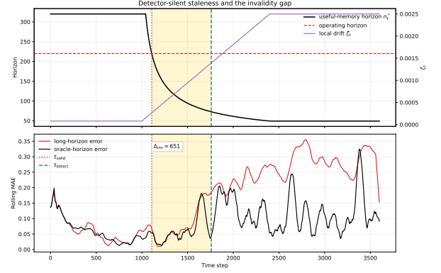
Figure 8: Temporal validity can fail before detector alarm. As drift intensifies, the temporal-validity horizon contracts until the operating horizon becomes stale at t_{\text{valid}} ; the detector responds only later at t_{\text{detect}} , leaving a strictly positive validity-detection lag. The lower panel shows excess tracking error accumulating before the alarm appears.
