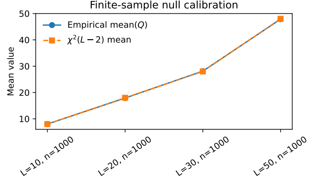
Figure 1: Finite-sample behavior of the oracle residual law.
