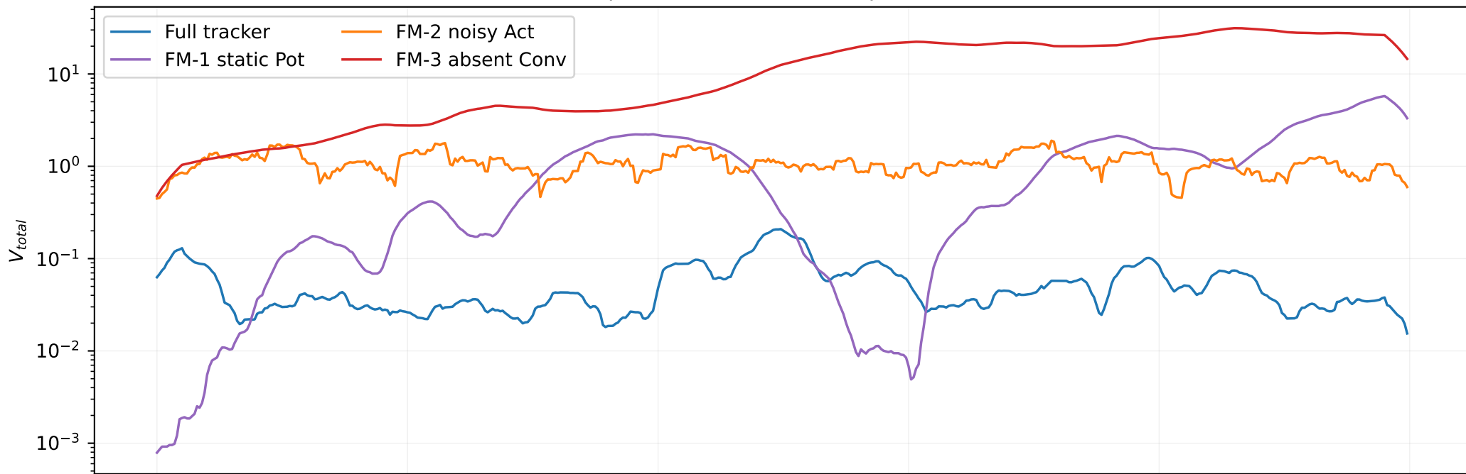
Component ablation under passive drift
