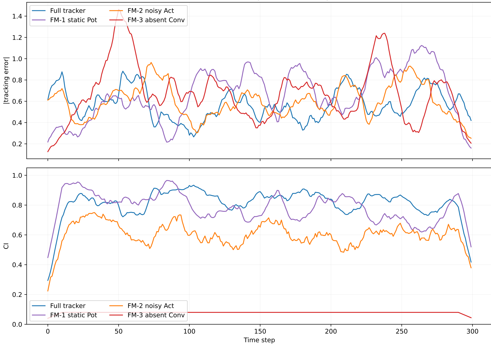
Particle-tracker ablation: rolling absolute tracking error and CI
