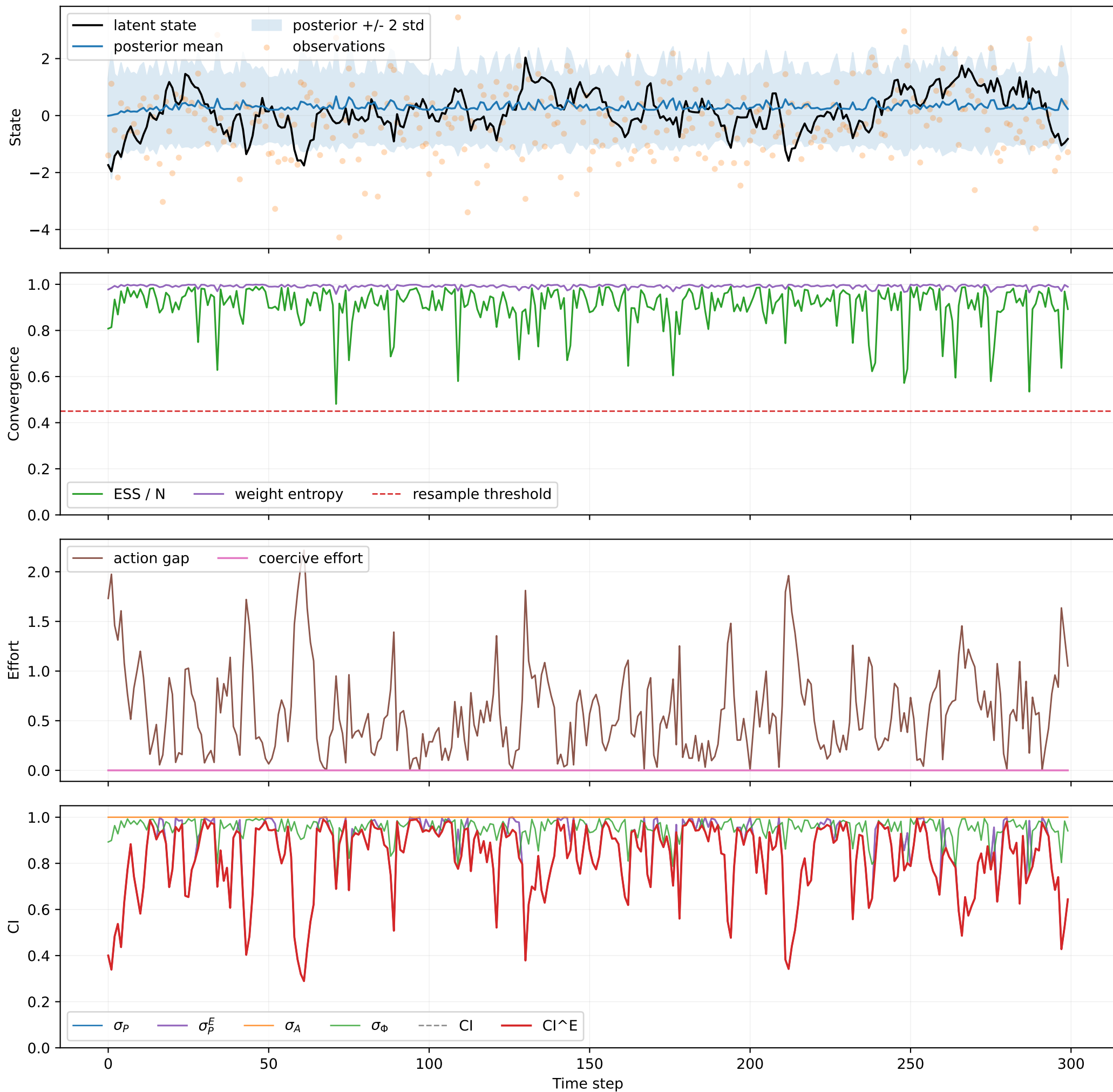
Triadic Particle Tracker: Full tracker (influence=0.00)
