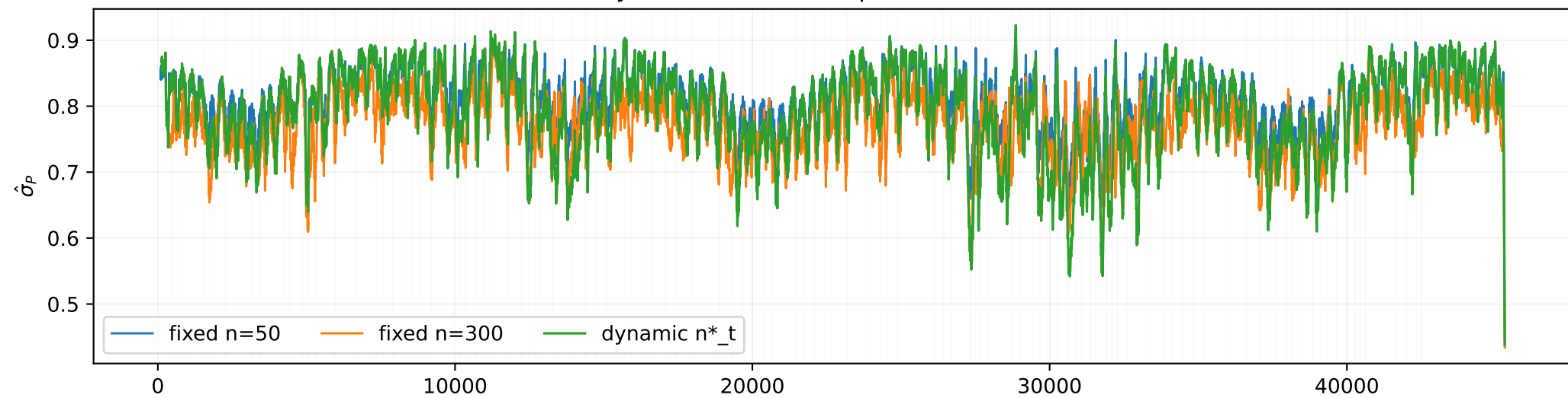
Dynamic window adaptation on ELEC2
