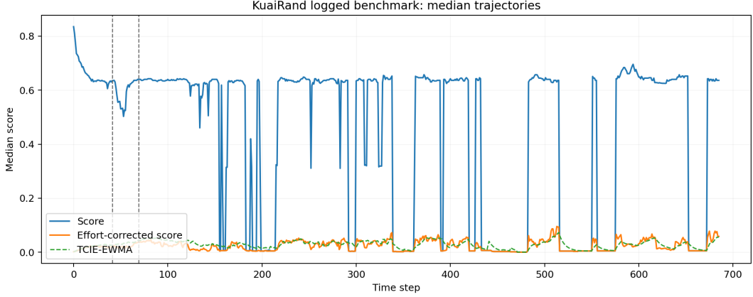
Figure 7: KuaiRand proxy-level logged benchmark. The random-exposure phase is treated as healthy, the first half of the later standard-recommendation slice as bubble formation, and the second half as collapse. Thresholds for CI, CI^E , and EWMA-smoothed CI^E are calibrated only on healthy windows.
