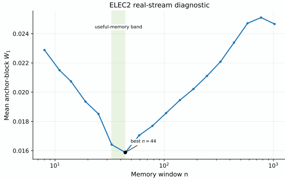
Figure 7: ELEC2 real-stream diagnostic on the nswprice marginal. The mean anchor-block W_1 error exhibits a finite interior optimum and a near-optimal useful-memory band, matching the temporal-validity signature on a real stream.
