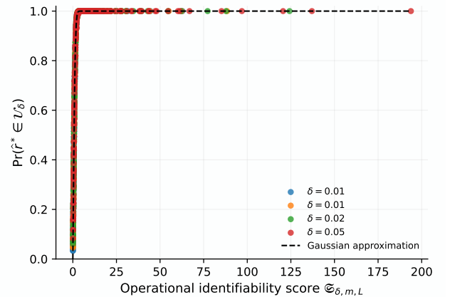
Figure 3: Operational identifiability of the useful-memory region. Across the tested grid, useful-region hit rates collapse against the score \mathfrak{S}_{\delta,m,L} = \sqrt{\mathcal{I}_{m,L}(H)} r_\delta(a, H) / \tau(H, \zeta) , matching the Gaussian approximation from Theorem 3.3.
