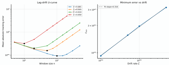
Figure 4: Interior risk optimum over memory length. Tracking error first falls with horizon and then rises once staleness overtakes the remaining variance gain. The optimum remains finite across drift strengths.
