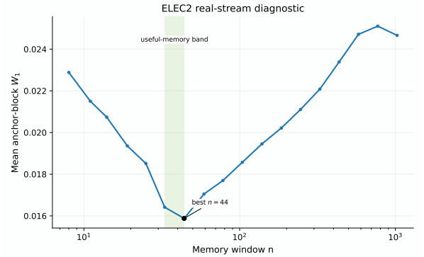
Figure 6: ELEC2 real-stream diagnostic on the nswwprice marginal. The mean anchor-block W_1 error exhibits a finite interior optimum and a near-optimal useful-memory band, matching the temporal-validity signature on a real stream.
