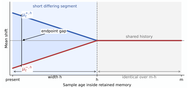
Figure 2: Least-favorable Gaussian path pair for the root- n horizon lower bound. The two paths share most of the retained history and differ only on a recent segment of width h , yet remain separated at the present. That recent segment already produces the same horizon exponent as the upper law in the root- n regime.
