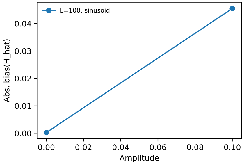
Regularity bias under misspecification
