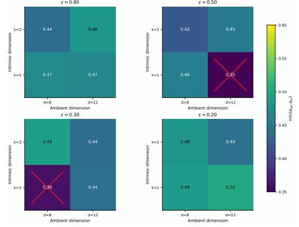
Figure 5: Empirical shape relevant to the bandwise fixed- \varepsilon Sinkhorn conjecture. Each panel reports the minimum of the i.i.d. and triangular finite-sample exponents over the ambient/intrinsic pairs tested at one regularization level. Crossed cells mark settings that fail the usefulness criterion. The resulting picture has a stable core and a small mixed boundary region on the tested grid.
