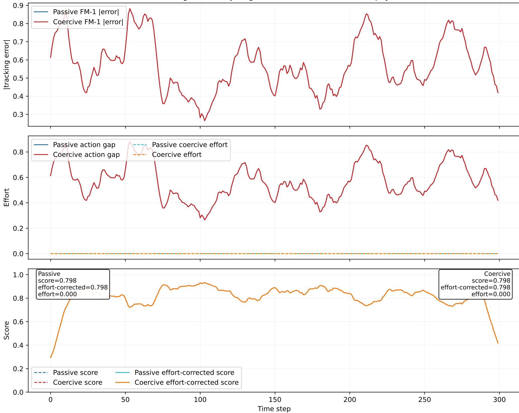
Coercive masking: score stays high while effort-corrected score pays for effort
