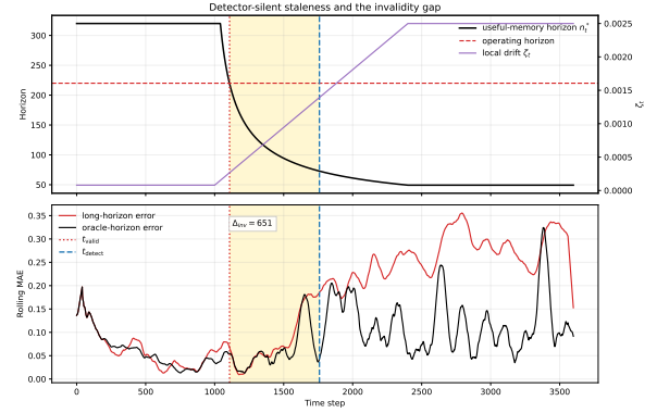
Figure 5: Temporal validity can fail before detector alarm. As drift intensifies, the temporal-validity horizon contracts until the operating horizon becomes stale at t_{\text{valid}} ; the detector responds only later at t_{\text{detect}} , leaving a strictly positive validity-detection lag. The lower panel shows excess tracking error accumulating before the alarm appears.
