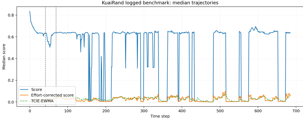
Figure 11: KuaiRand proxy-level logged benchmark. The random-exposure phase is treated as healthy, the first half of the later standard-recommendation slice as bubble formation, and the second half as collapse. Thresholds for CI, CI^E , and EWMA-smoothed CI^E are calibrated only on healthy windows.
