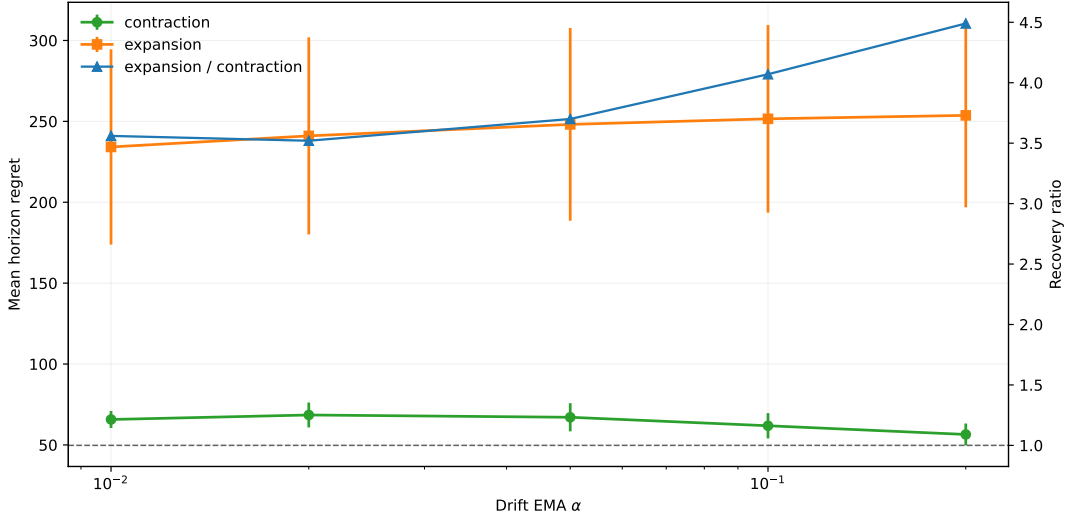
Figure 6: EMA sensitivity of horizon recovery on alternating timescales. The drift-EMA coefficient changes how quickly the regulator reacts to bursts, but the asymmetry remains: expansion regret stays above contraction regret across the sweep, and the ratio is larger at higher \alpha in this benchmark.
