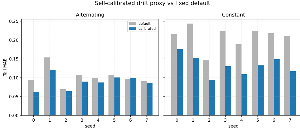
Figure 9: Prefix-validated self-calibration of the drift proxy. The selected (d, \alpha) shifts the operating point of the regulator; on this calibration study it improves tail MAE relative to the fixed default.
