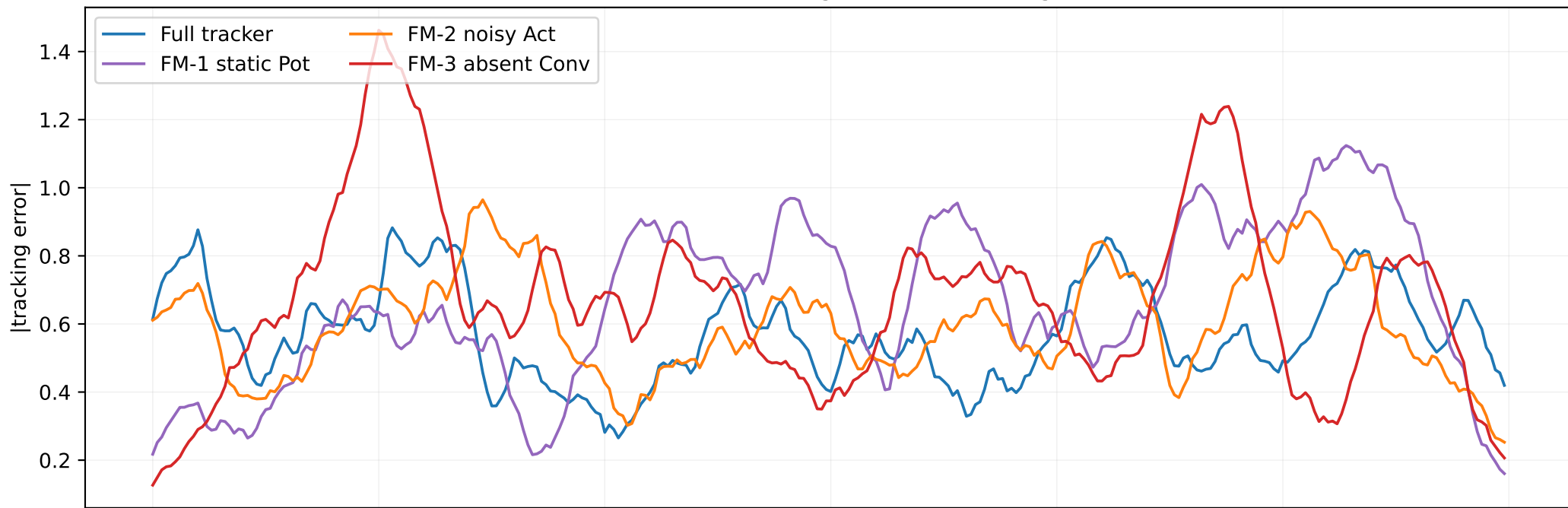
Particle-tracker ablation: rolling absolute tracking error and CI
