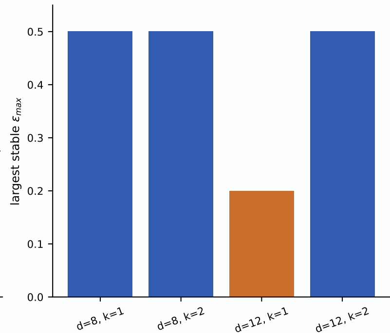
Maximal stable epsilon band
