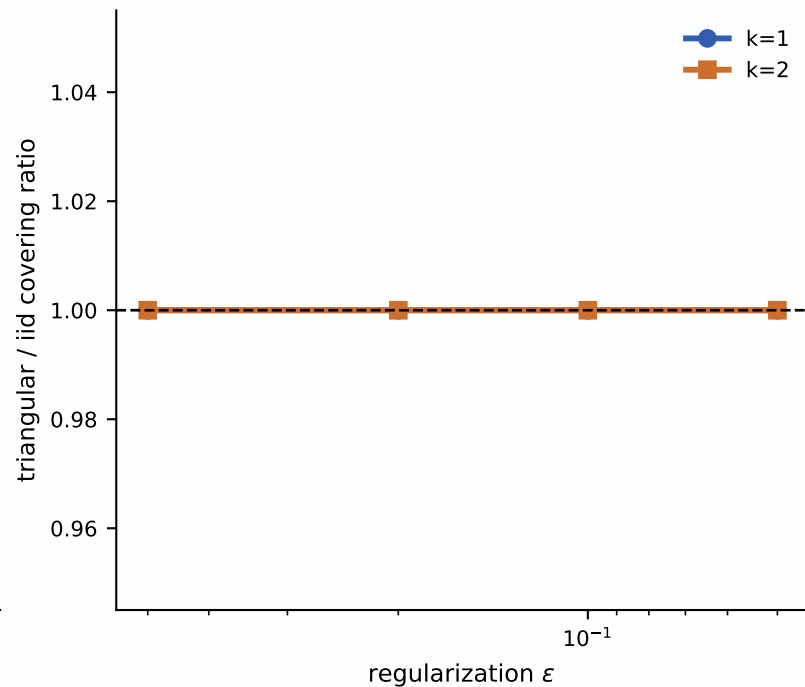
Exact support-complexity inheritance
