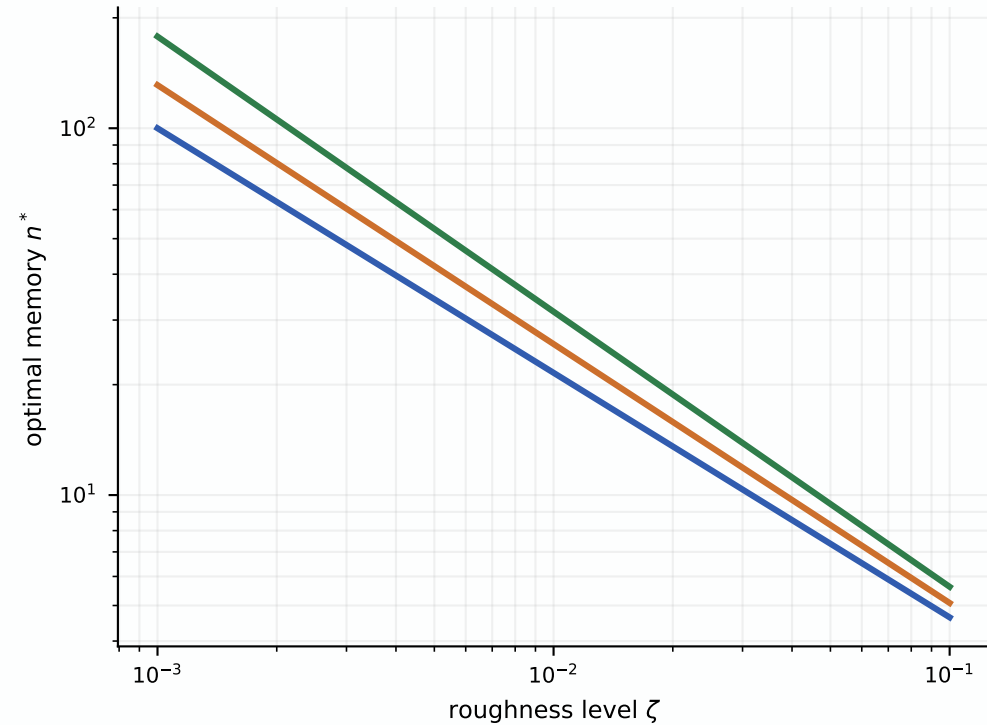
Prescriptive horizon law
