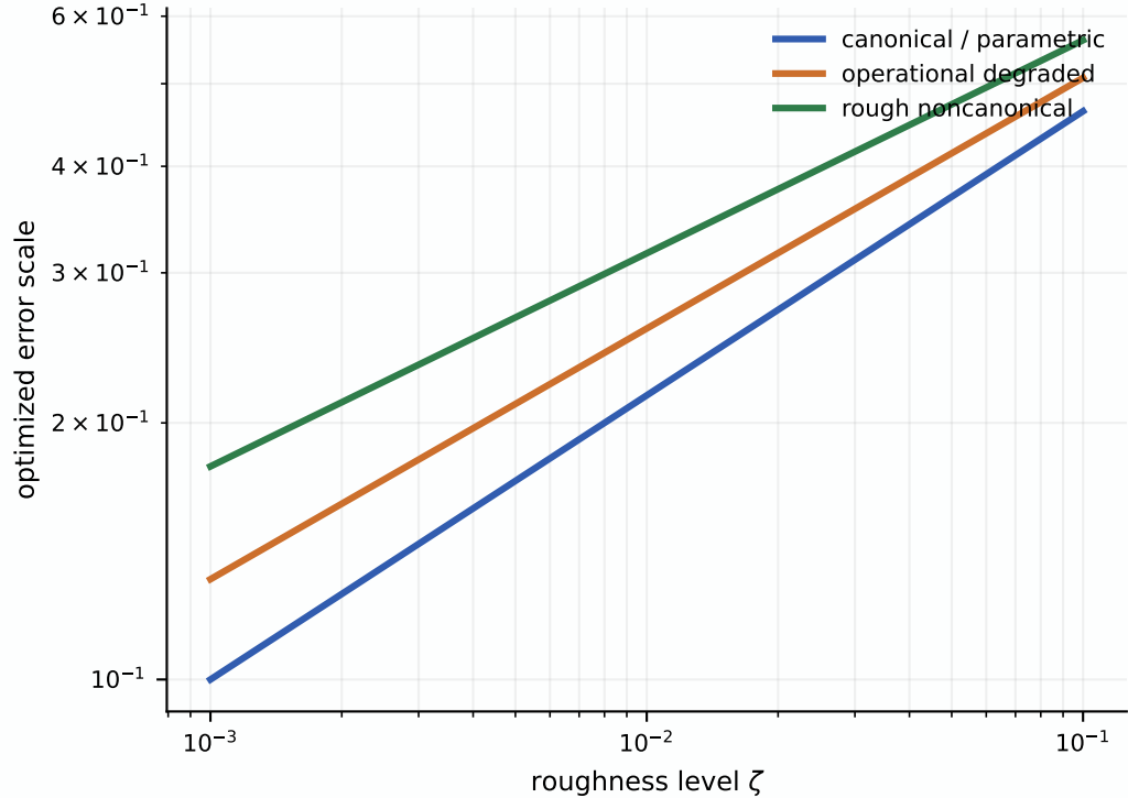
Prescriptive error law
