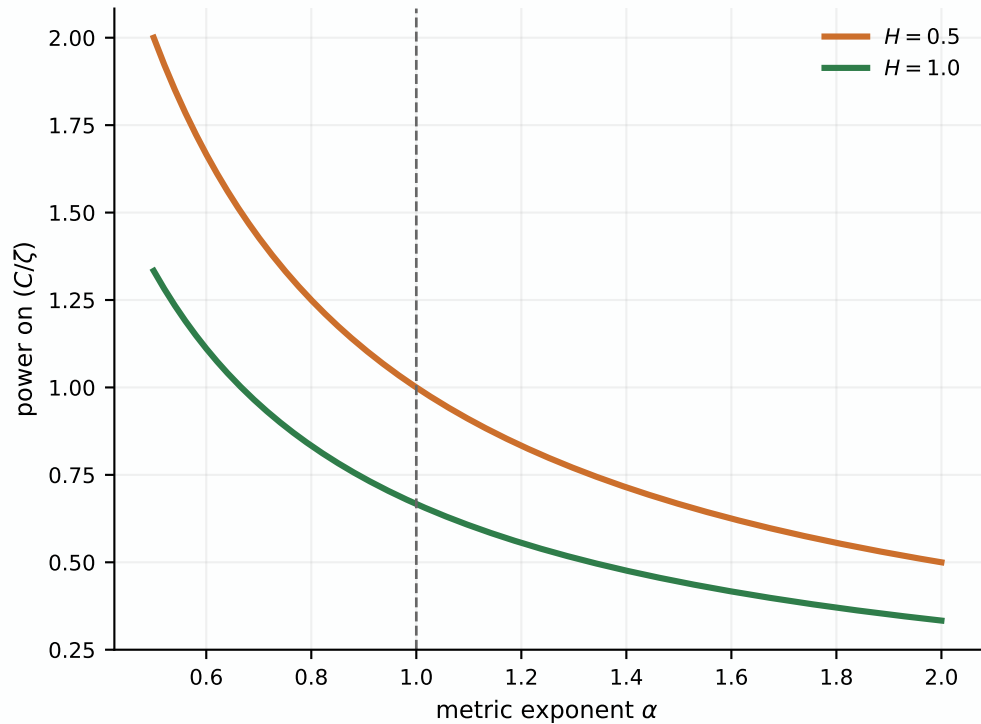
Horizon exponent 1/[\alpha(1/2 + H)]
