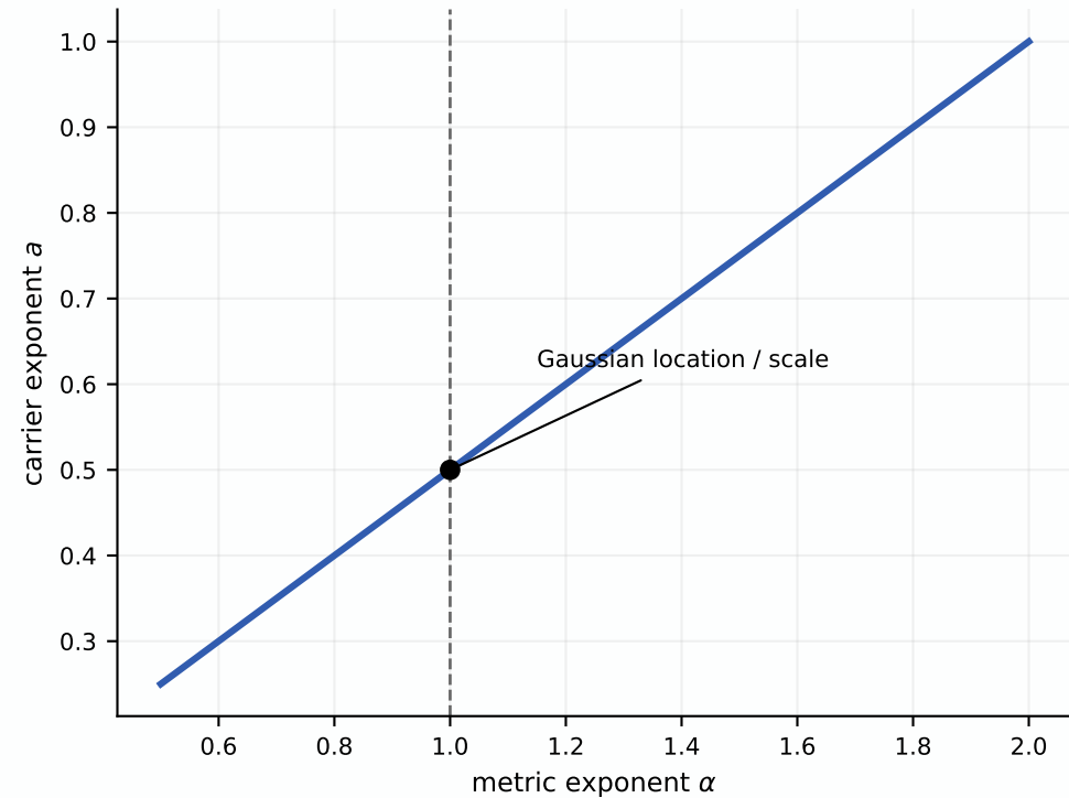
Carrier exponent a = \alpha/2
