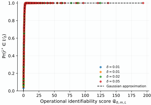
Figure 3: Operational identifiability of the useful-memory region. Across the tested grid, useful-region hit rates collapse against the score \mathcal{S}_{\delta,m,L} = \sqrt{\mathcal{I}_{m,L}(H)} r_\delta(a, H) / \tau(H, \zeta) , matching the Gaussian approximation from Theorem 4.3.
