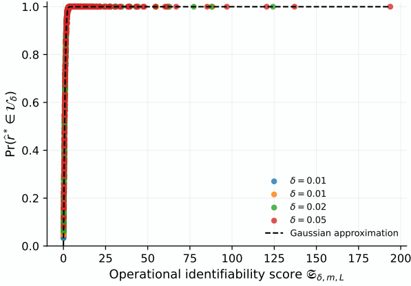
Figure 3: Operational identifiability of the useful-memory region. Across the tested grid, useful-region hit rates collapse against the score \mathfrak{S}_{\delta,m,L} = \sqrt{\mathcal{I}_{m,L}(H)}r_\delta(a, H)/\tau(H, \zeta) , matching the Gaussian approximation from Theorem 3.3.
