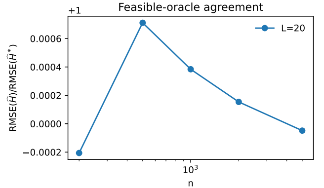
Figure 3: Feasible-oracle agreement for estimation of H .
