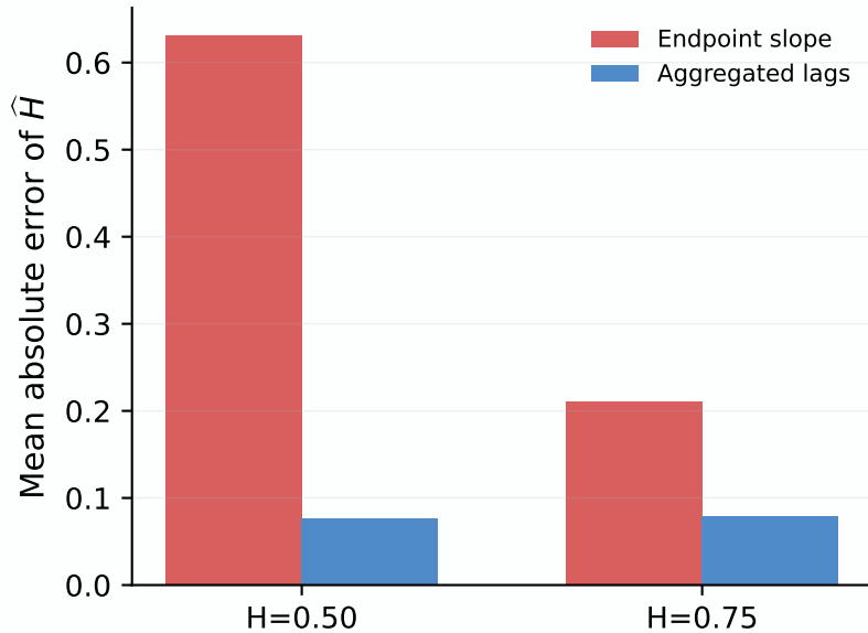
Roughness estimation with \hat{k} \approx 1
