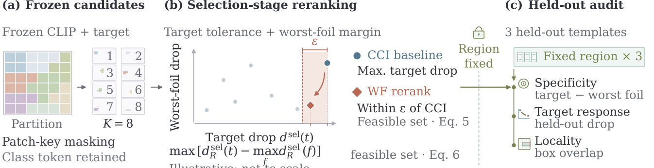
Figure 1: Selection and held-out audit. A region is fixed using selection-stage responses before three-template evaluation of specificity, target response, and locality. Schematic responses illustrate the selection rule.
