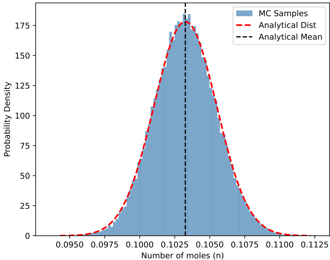
Distribution of n (correlated)
