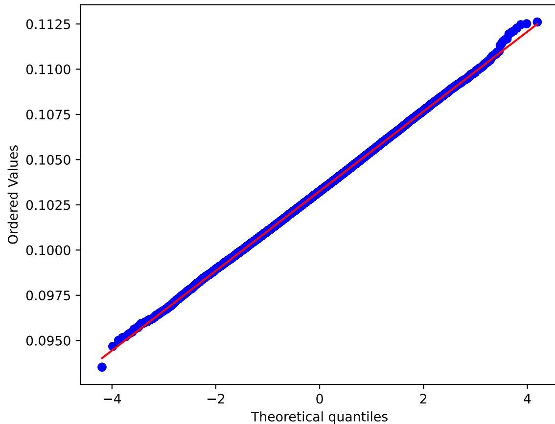
Q-Q Plot (correlated)
