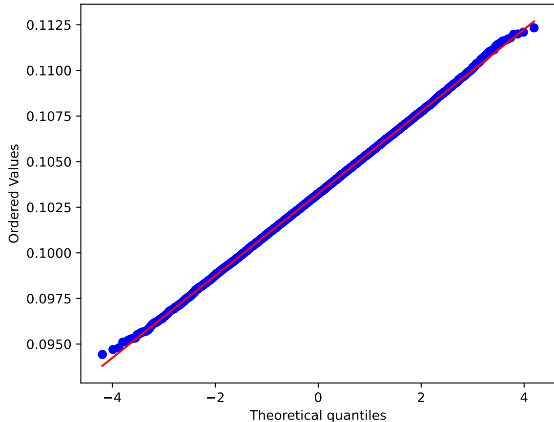
Q-Q Plot (independent)
