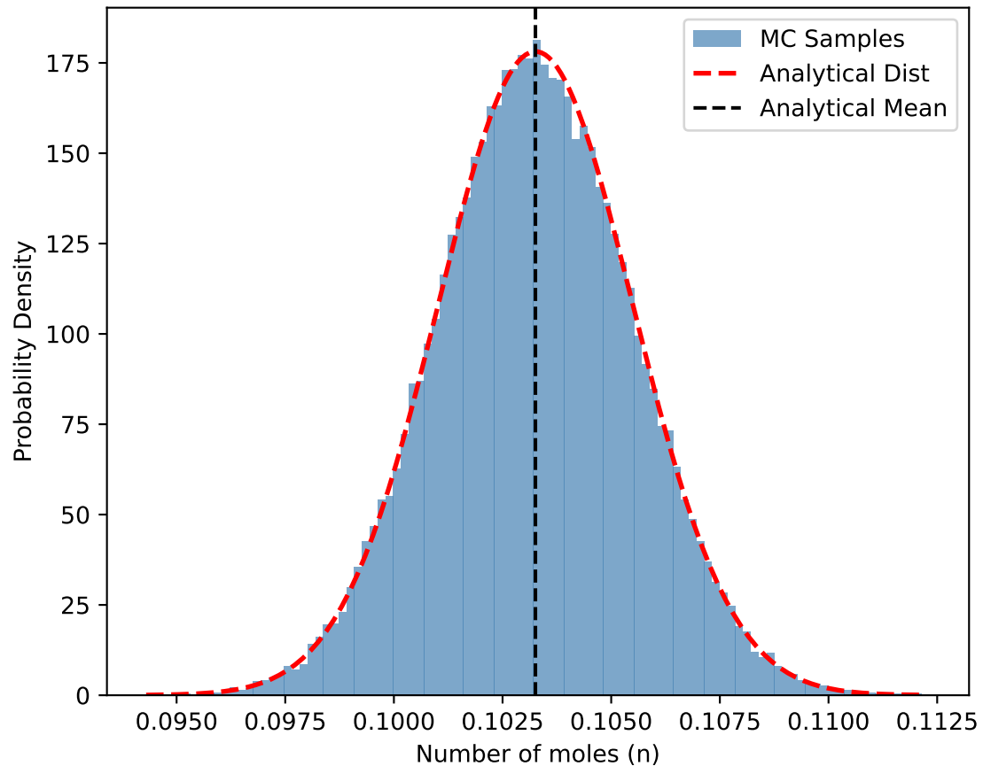
Distribution of n (independent)
