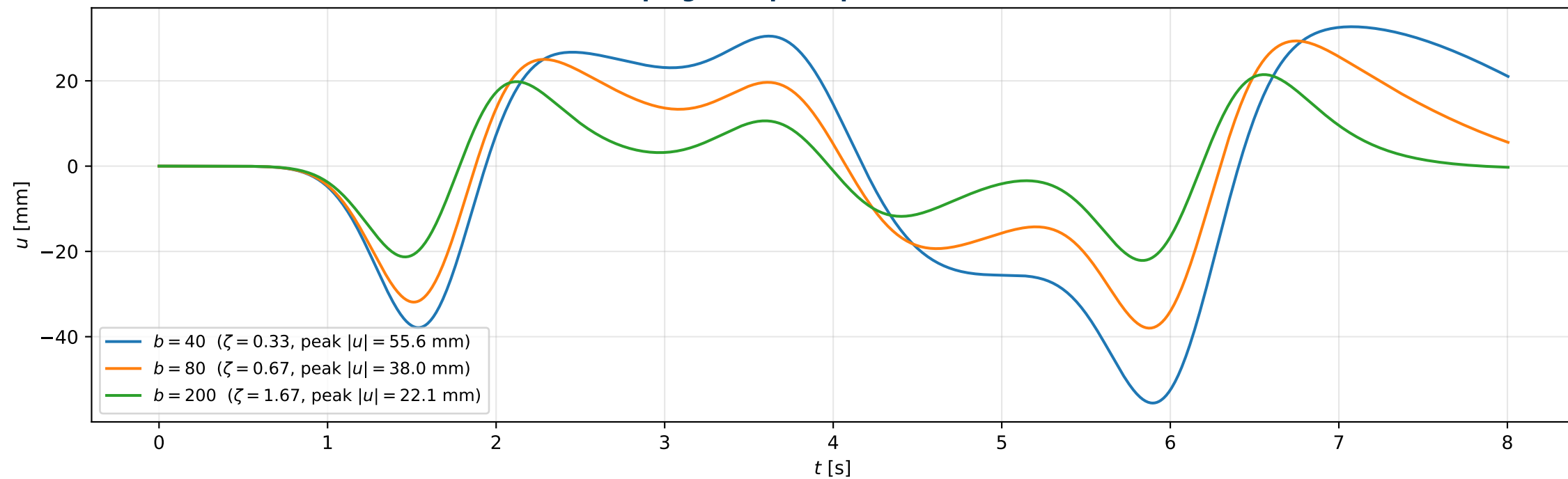
Damping sweep (displacement vs time)
