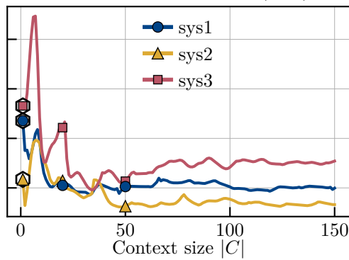
Decoder performance (loss)
