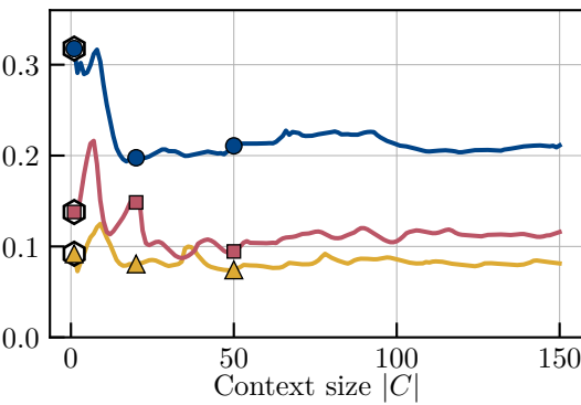
MSE of mean prediction
