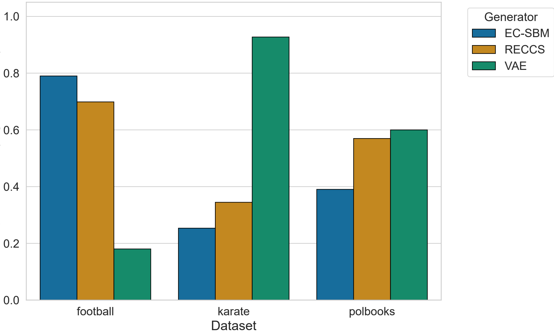
Composite Score (Higher is Better)
