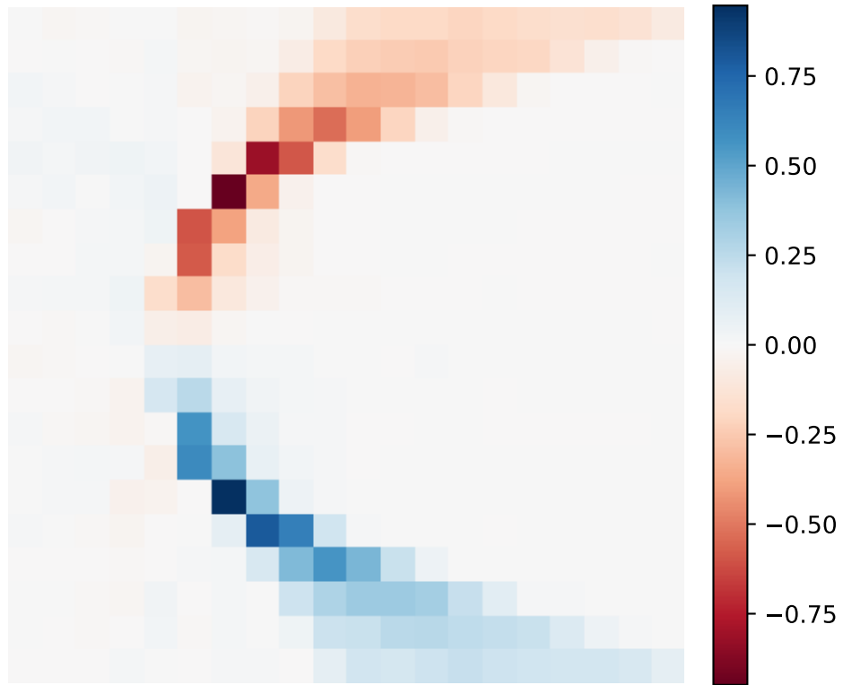
Finite difference - Slice 10
