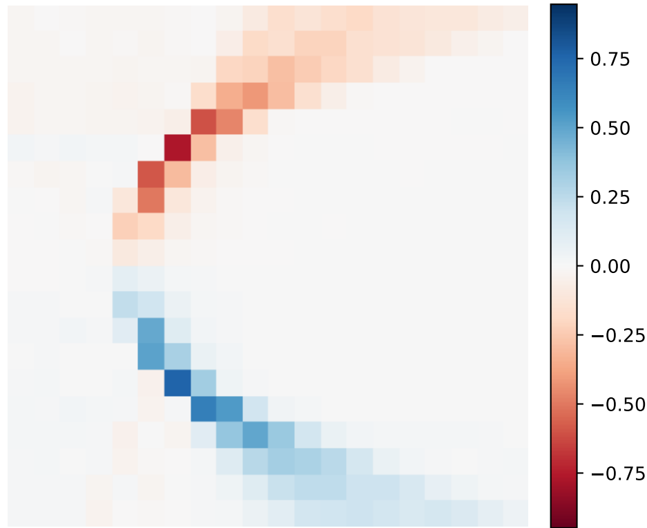
Automatic differentiation - Slice 10
